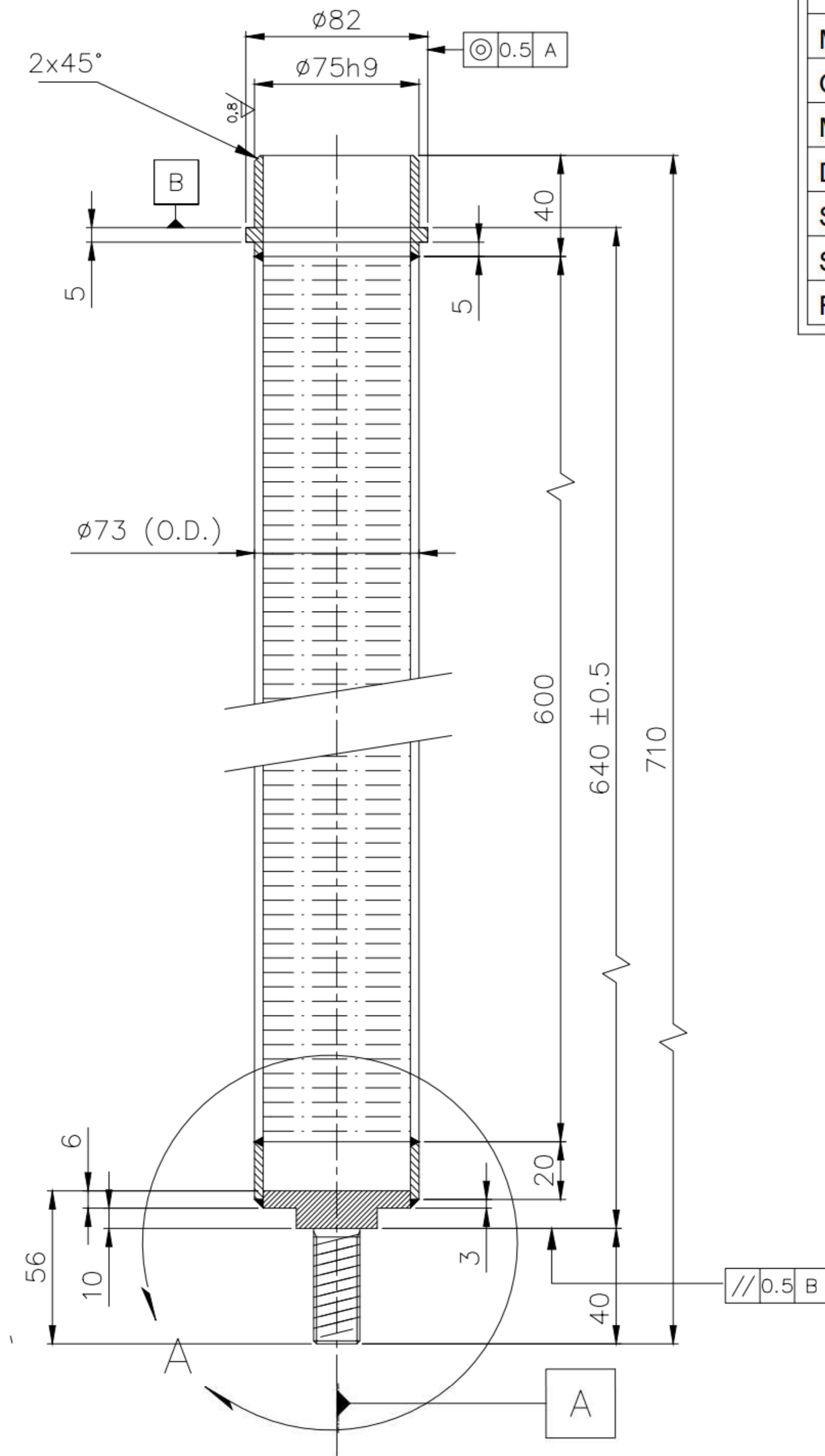
Wedge Wire Tube ( Cartridge)
