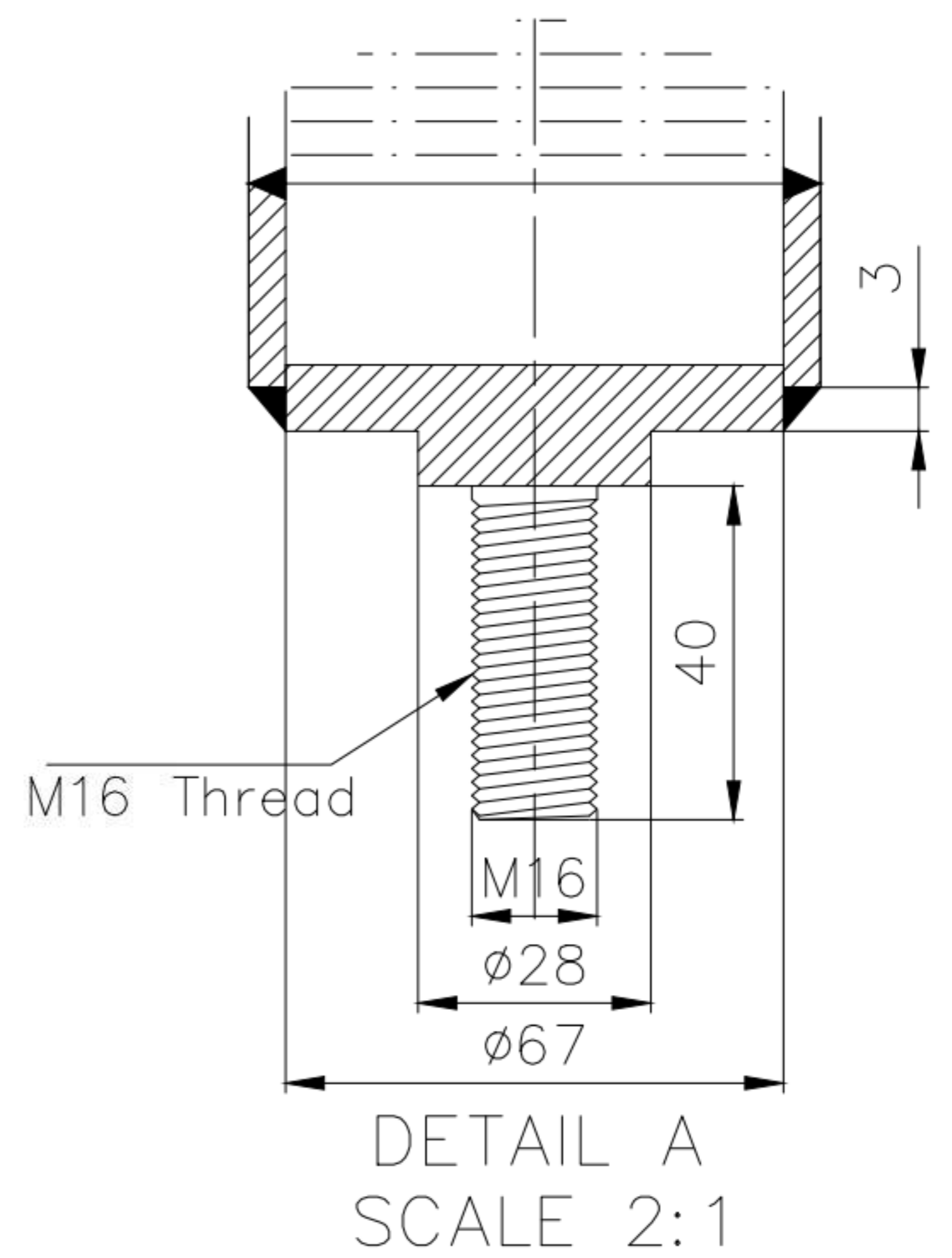
Wedge Wire Tube ( Cartridge)
